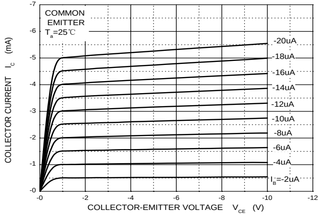
Static Characteristic
