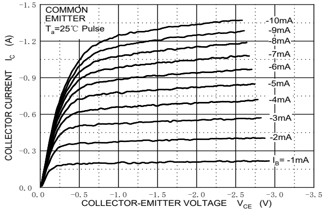
Static Characteristic
