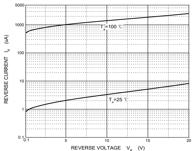
Reverse Characteristics
