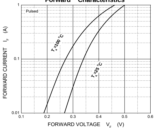
Forward Characteristics
