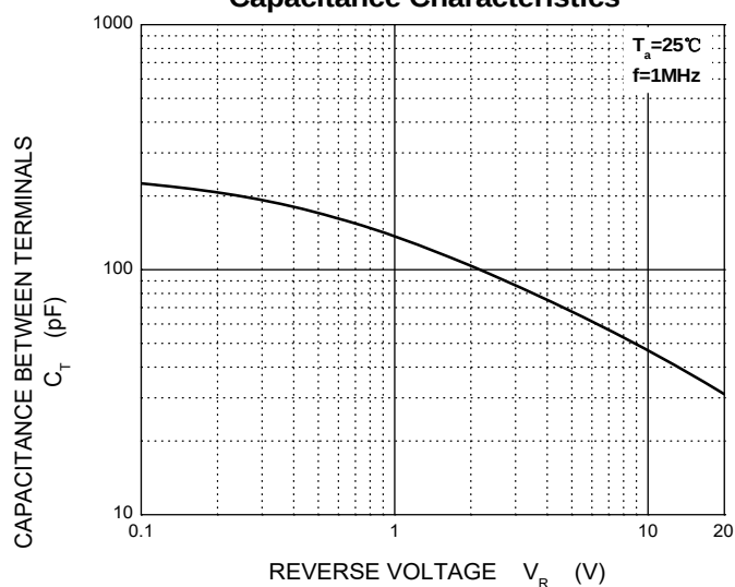
Capacitance Characteristics
