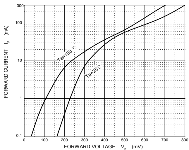
Forward Characteristics
